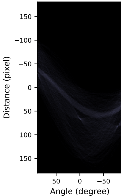
Hough transform
